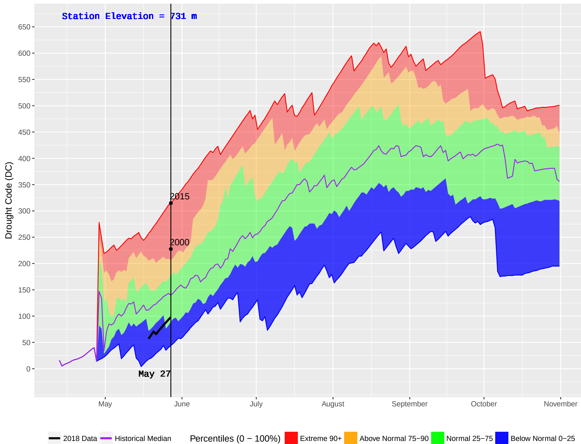
FIRESIDE (440) : Historical (1996–2016) and Current (2018) Noon Drought Code (DC)
