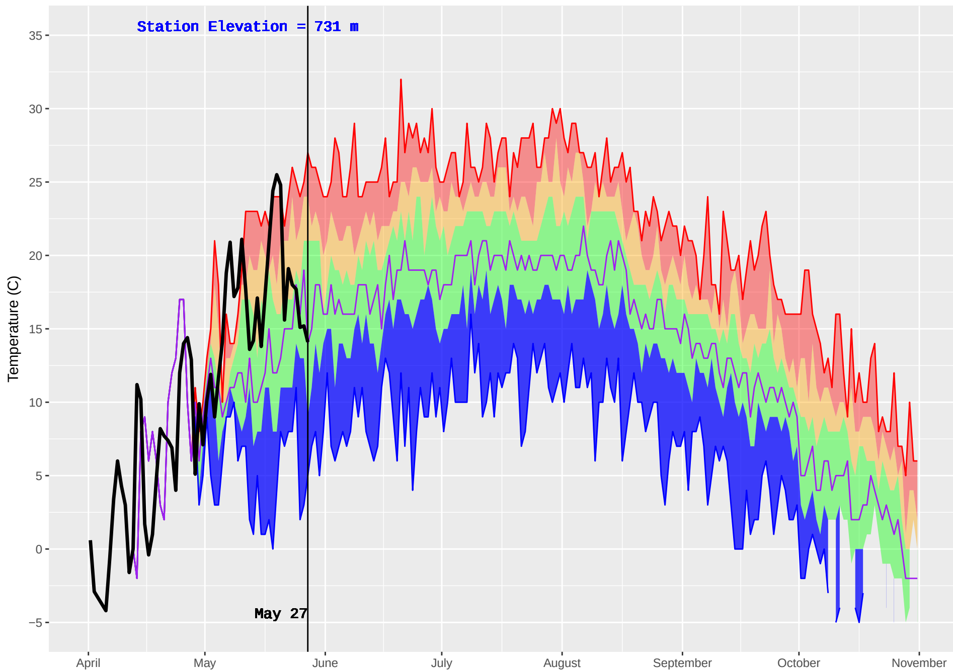
FIRESIDE (440) : Historical (1996–2016) and Current (2018) Noon Temperature
