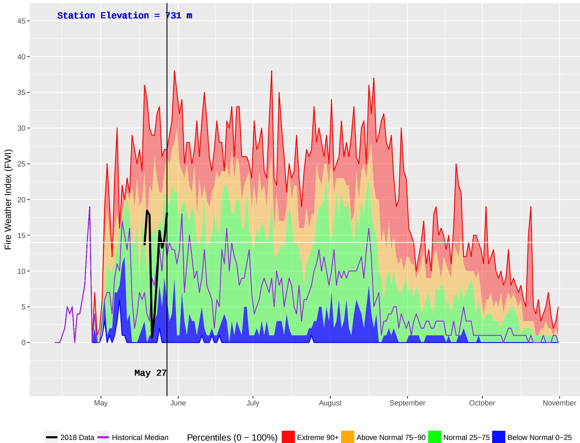
FIRESIDE (440) : Historical (1996–2016) and Current (2018) Noon Fire Weather Index (FWI)
