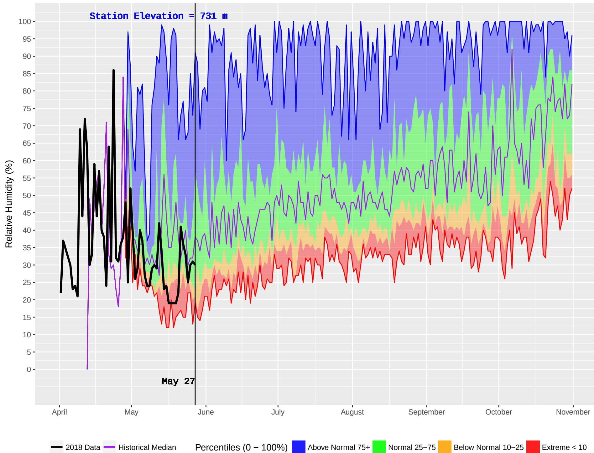
FIRESIDE (440) : Historical (1996–2016) and Current (2018) Noon Relative Humidity
