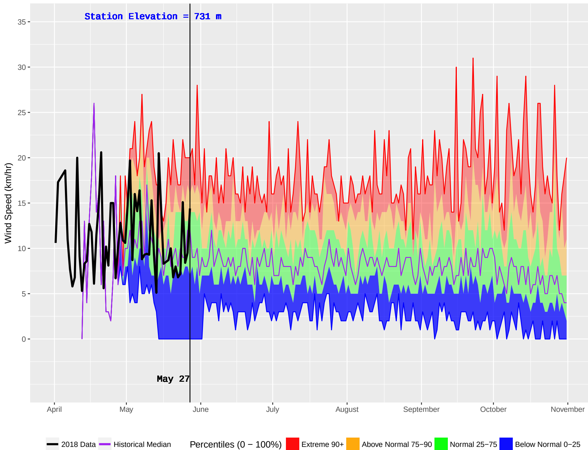
FIRESIDE (440) : Historical (1996–2016) and Current (2018) Noon Wind Speed
