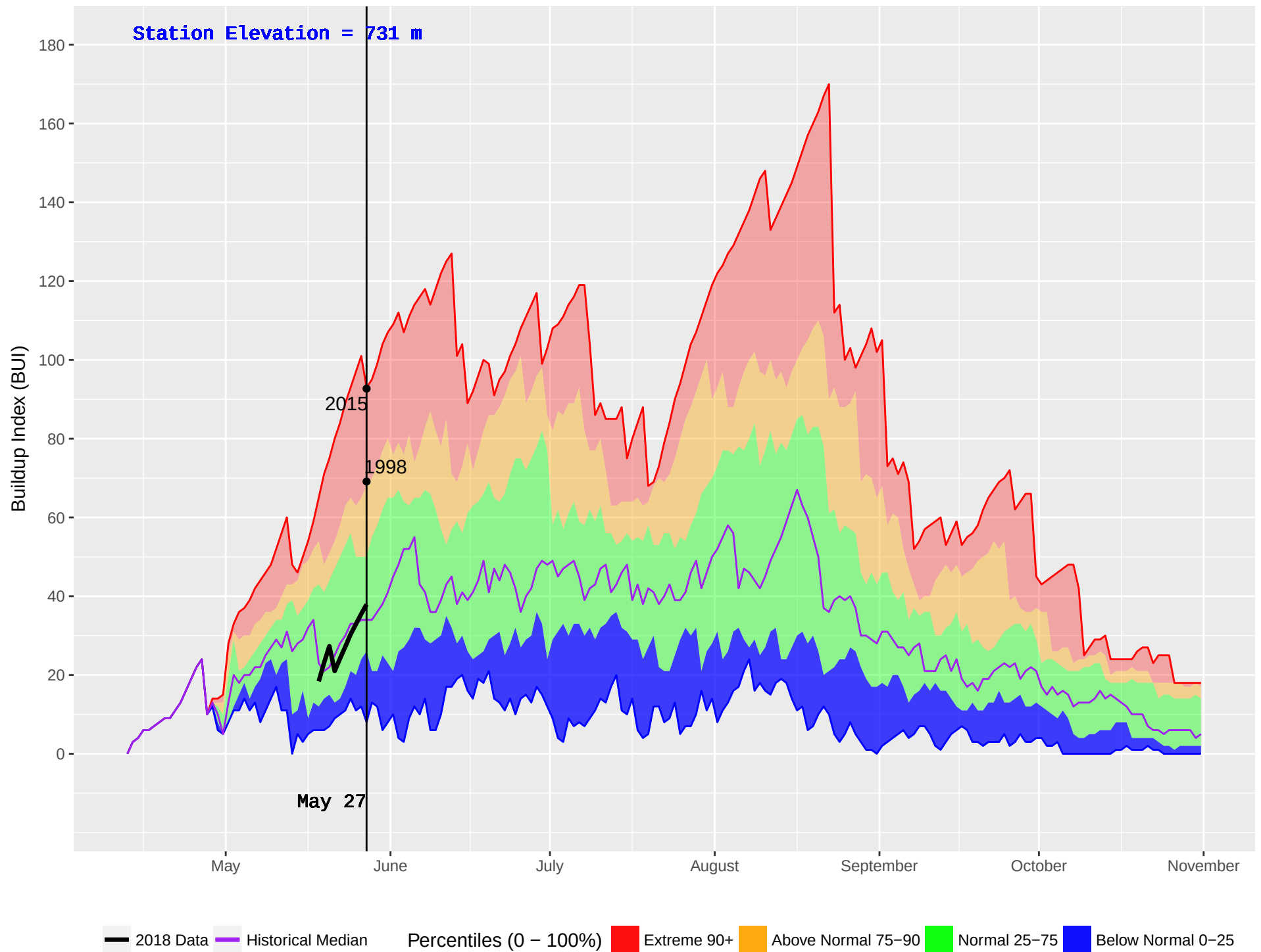
FIRESIDE (440) : Historical (1996–2016) and Current (2018) Noon Buildup Index (BUI)
