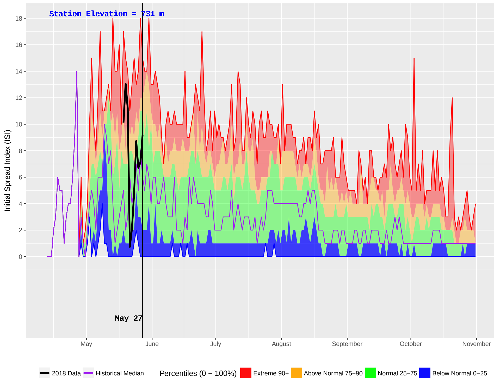
FIRESIDE (440) : Historical (1996–2016) and Current (2018) Noon Initial Spread Index (ISI)
